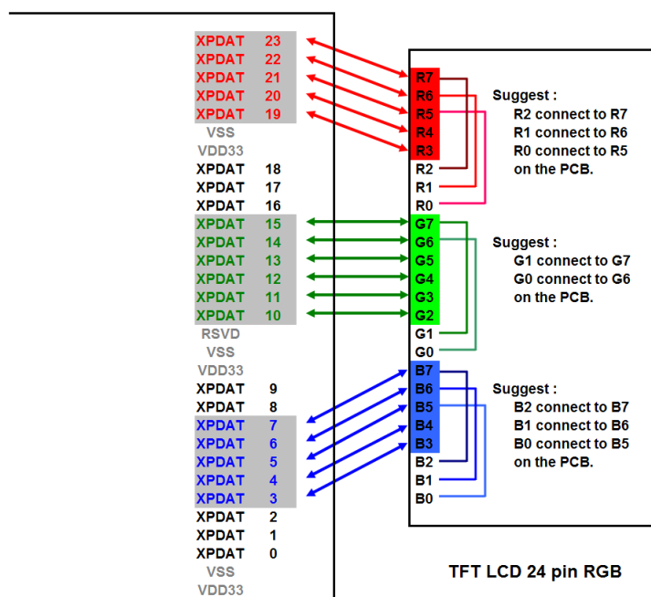
Figure 10-3 : RA8889 color depth 16bit with LCD panel pin connect
