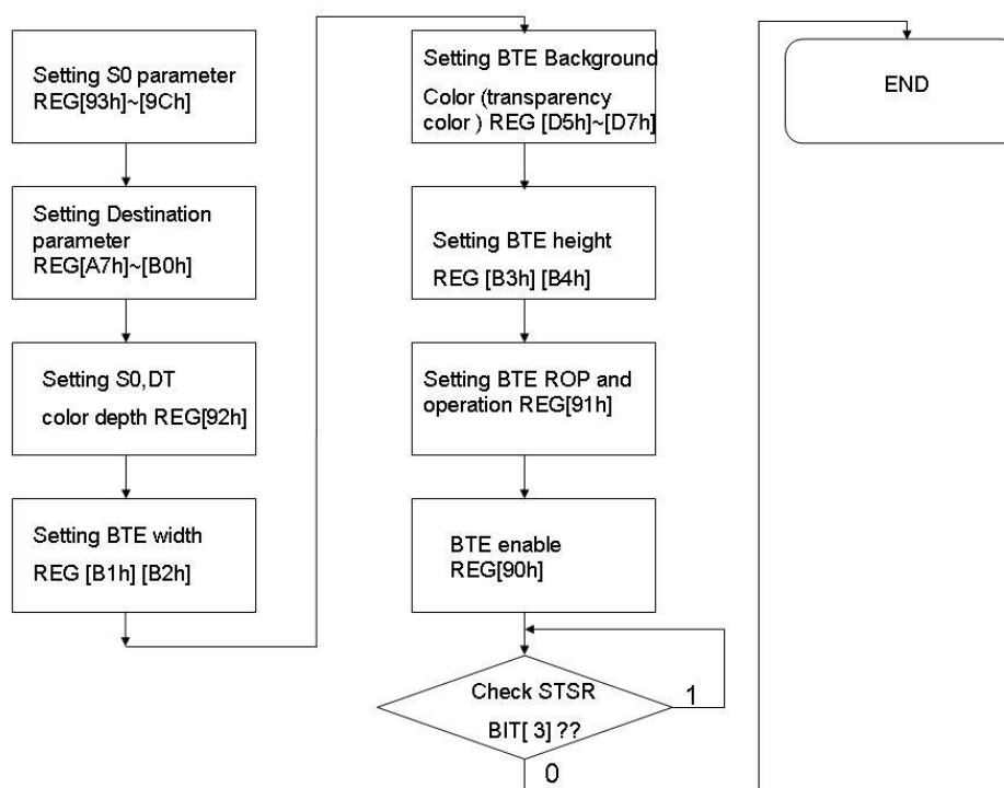
Figure 13-18 : Flow Chart
